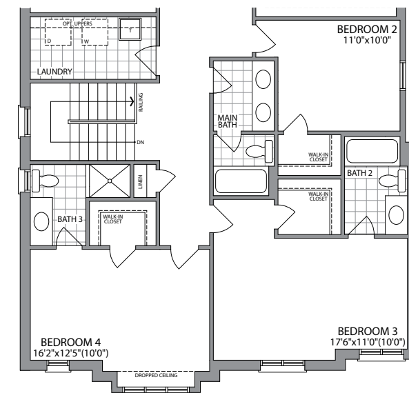
OPT. SECOND FLOOR W/5 BEDROOMS ELEVATION 2
