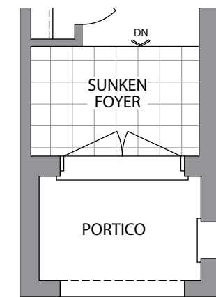
GROUND FLOOR ELEVATION 2
