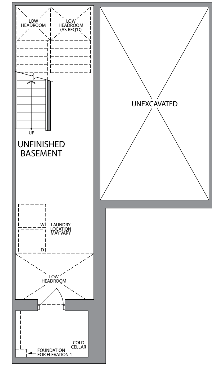
BASEMENT ELEVATION 1 & 2
