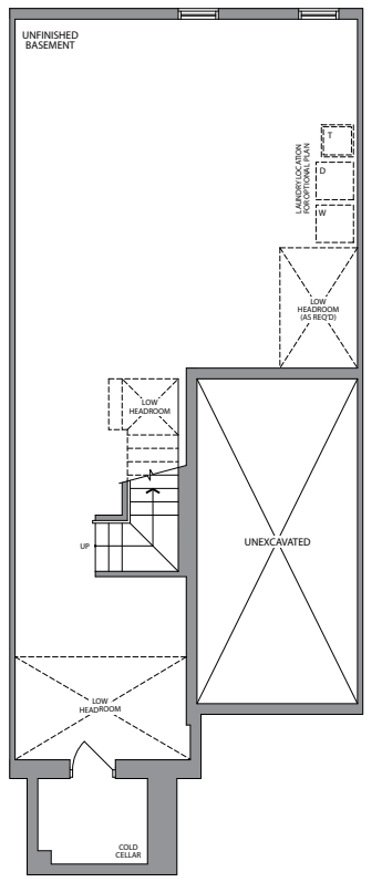
BASEMENT ELEVATION 1
