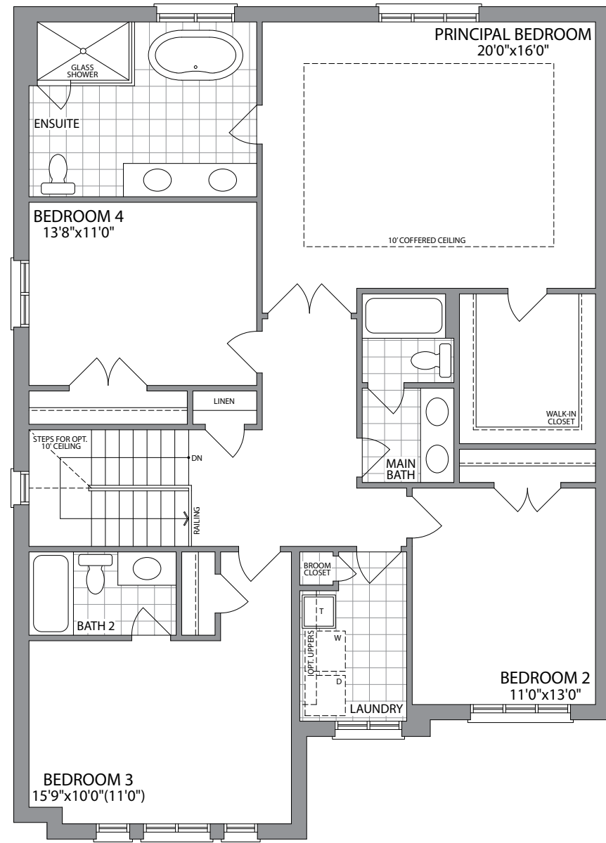
SECOND FLOOR ELEVATION 1
