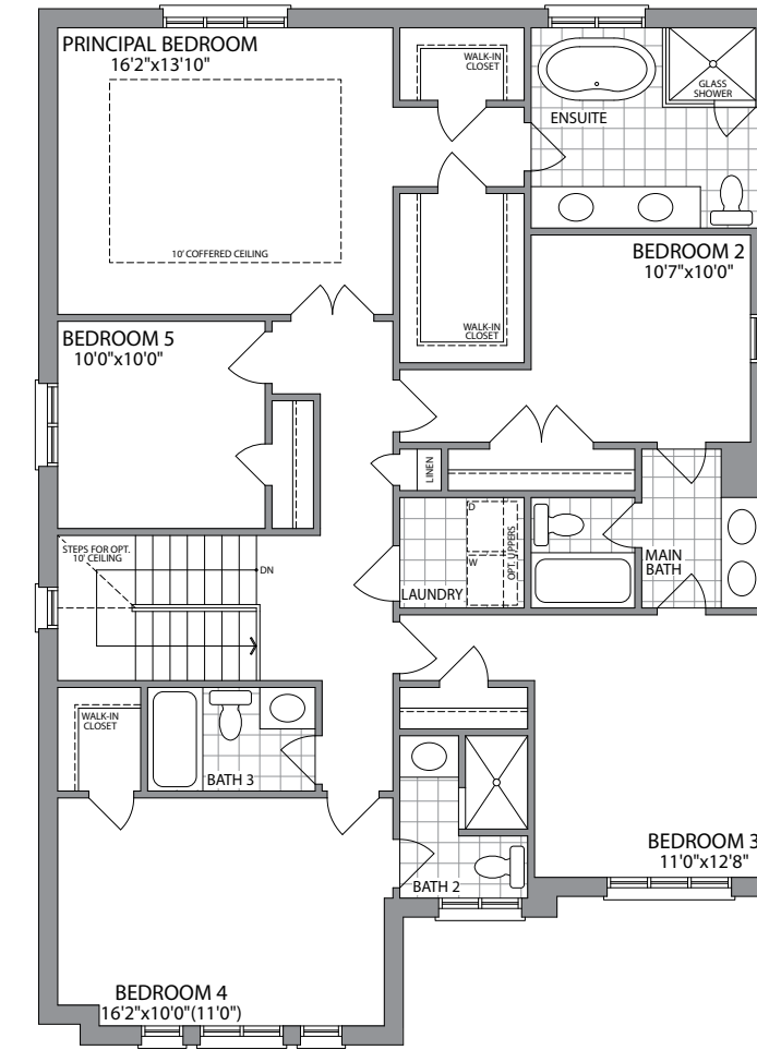
OPT. SECOND FLOOR W/5 BEDROOMS ELEVATION 1
