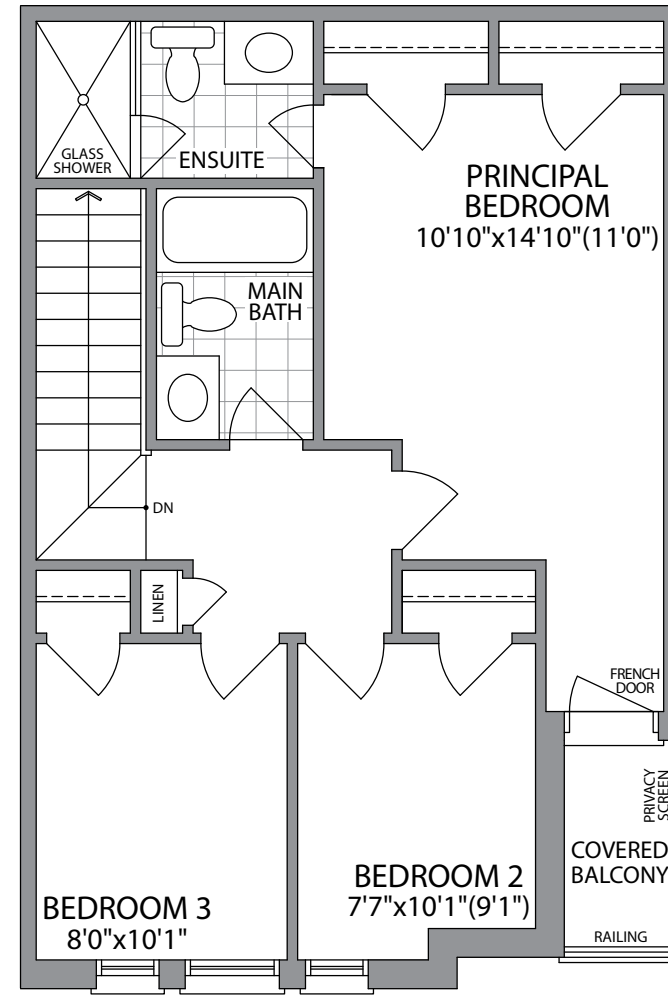
THIRD FLOOR ELEVATION 1 & 2
