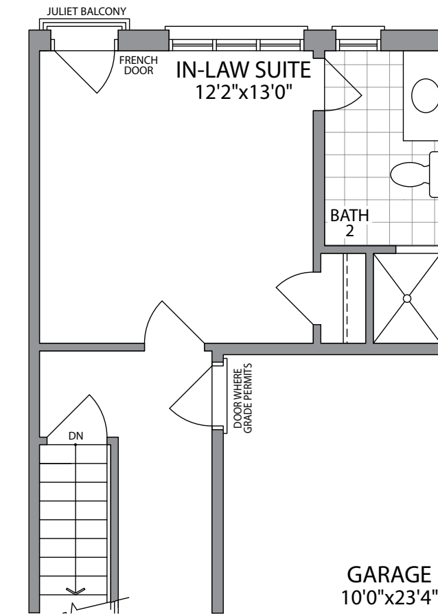
OPT. GROUND FLOOR W/IN-LAW SUITE ELEVATION 1 & 2
