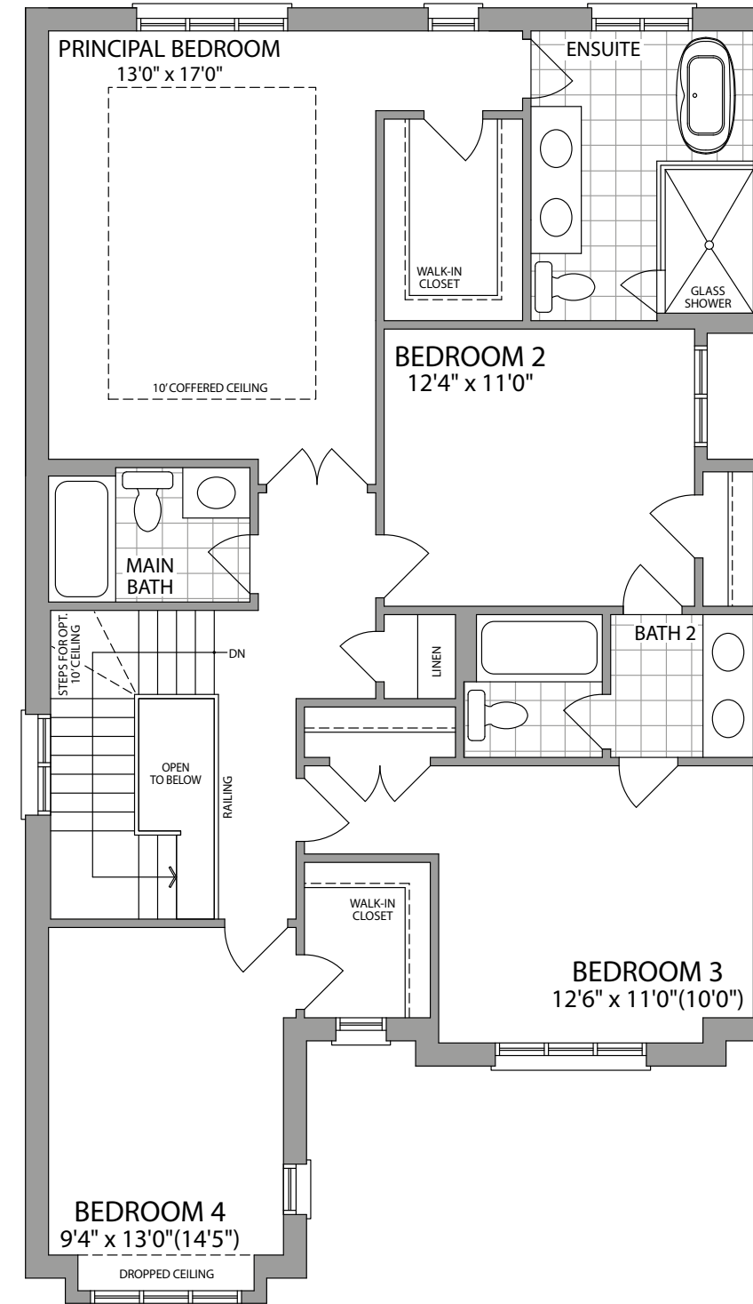
SECOND FLOOR ELEVATION 3
