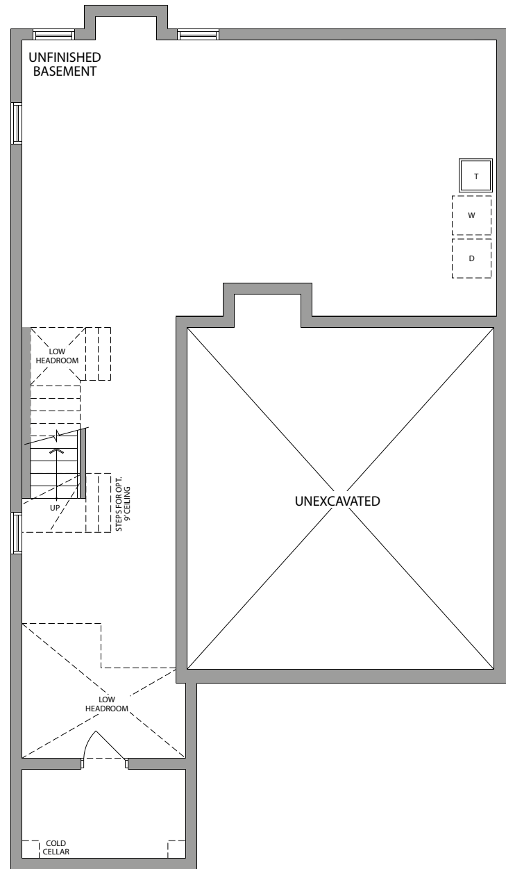
BASEMENT ELEVATION 3 & 2
