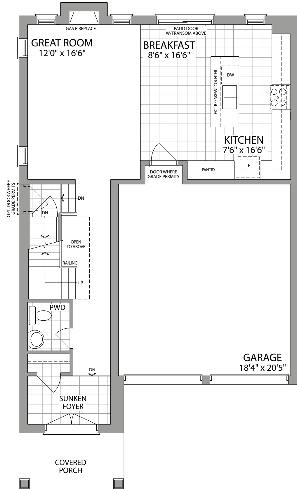
GROUND FLOOR ELEVATION 3
