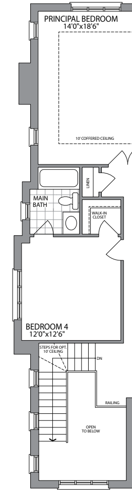
SECOND FLOOR ELEVATION 2C
