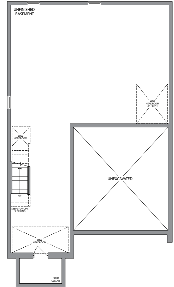
BASEMENT ELEVATION 1
