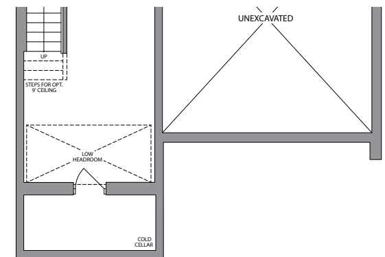
BASEMENT ELEVATION 2
