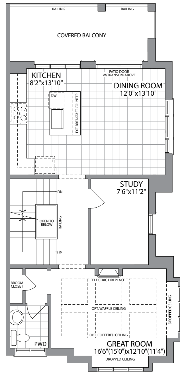
MAIN FLOOR ELEVATION 1C
