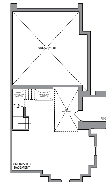
BASEMENT ELEVATION 1C
