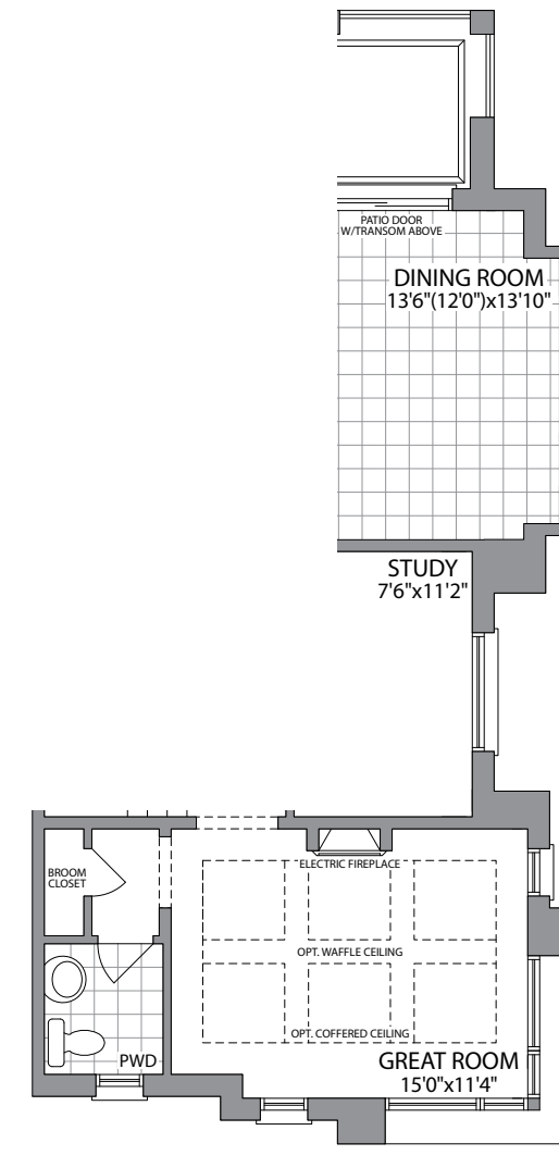
MAIN FLOOR ELEVATION 2C
