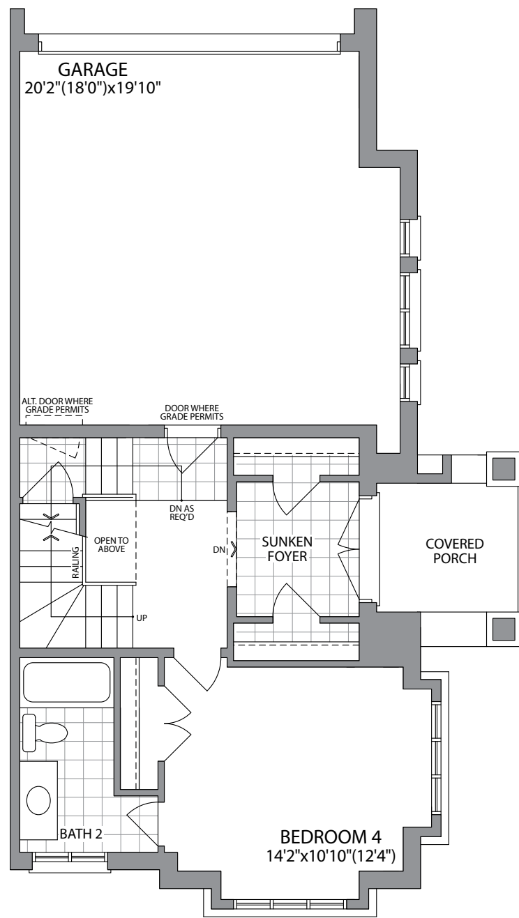
GROUND FLOOR ELEVATION 1C
