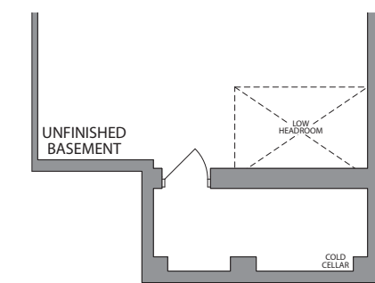
BASEMENT ELEVATION 2C
