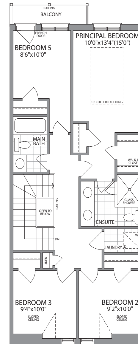
OPT. THIRD FLOOR W/5 BEDROOMS ELEVATION 1C
