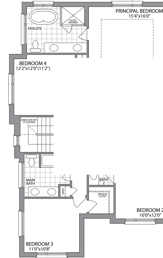
SECOND FLOOR ELEVATION 2C
