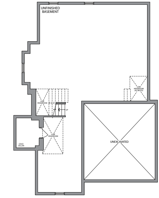
BASEMENT ELEVATION 1C
