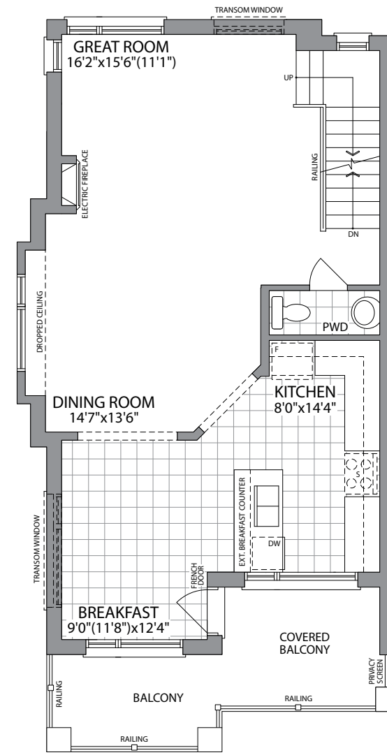
MAIN FLOOR ELEVATION 2C
