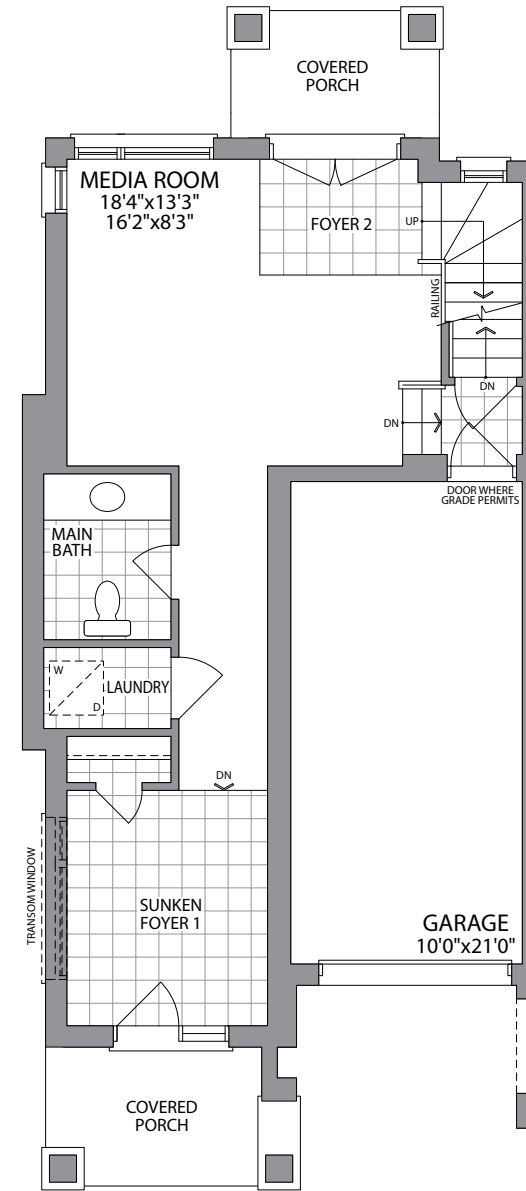
GROUND FLOOR ELEVATION 2C
