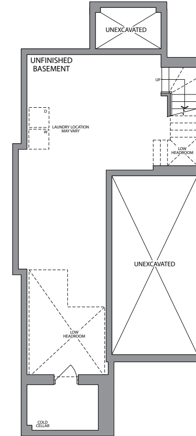
BASEMENT ELEVATION 1C & 2C
