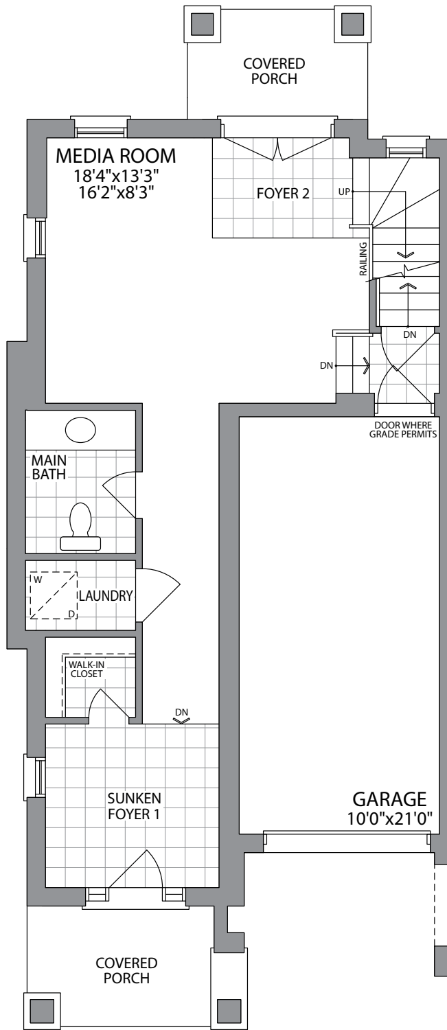
GROUND FLOOR ELEVATION 1C
