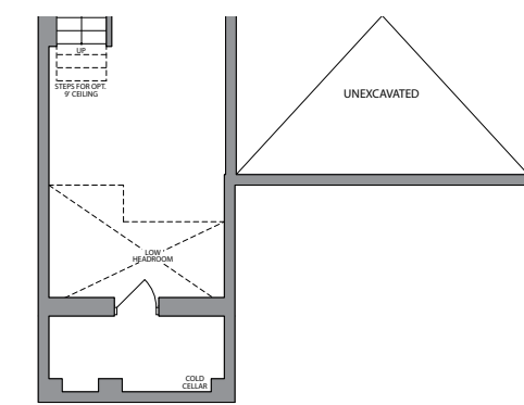
BASEMENT ELEVATION 2
