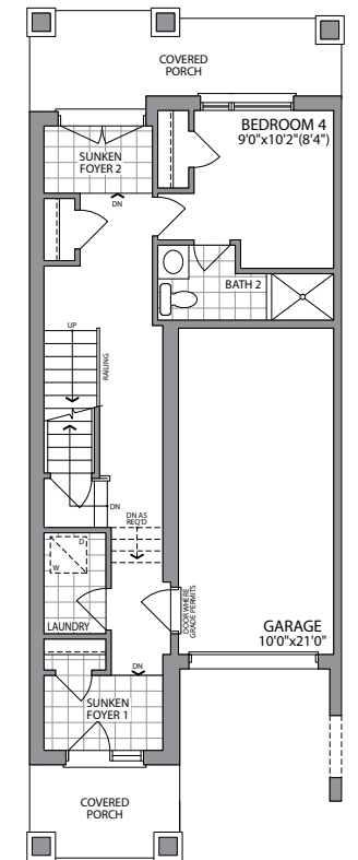
OPT. GROUND FLOOR W/4 BEDROOMS ELEVATION 2C
