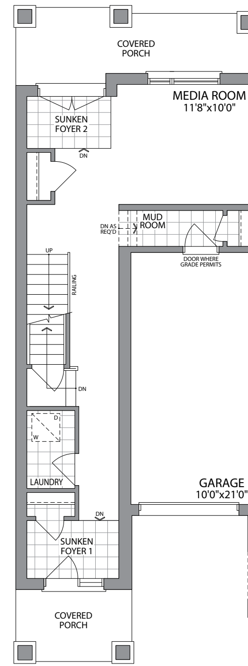
GROUND FLOOR ELEVATION 2C
