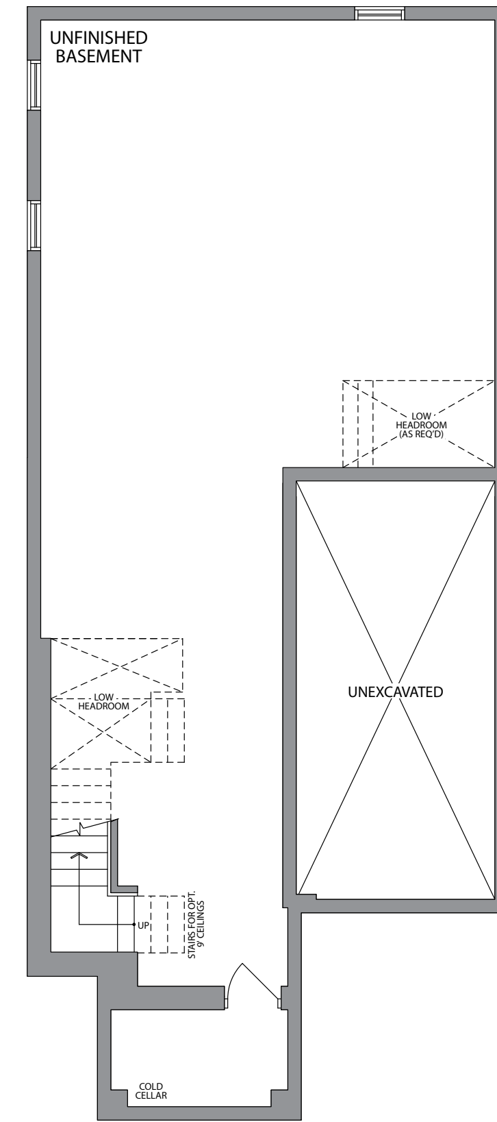
BASEMENT ELEVATION 1 & 2
