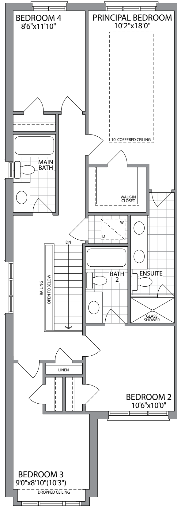
OPT. SECOND FLOOR W/4 BEDROOMS ELEVATION 1C
