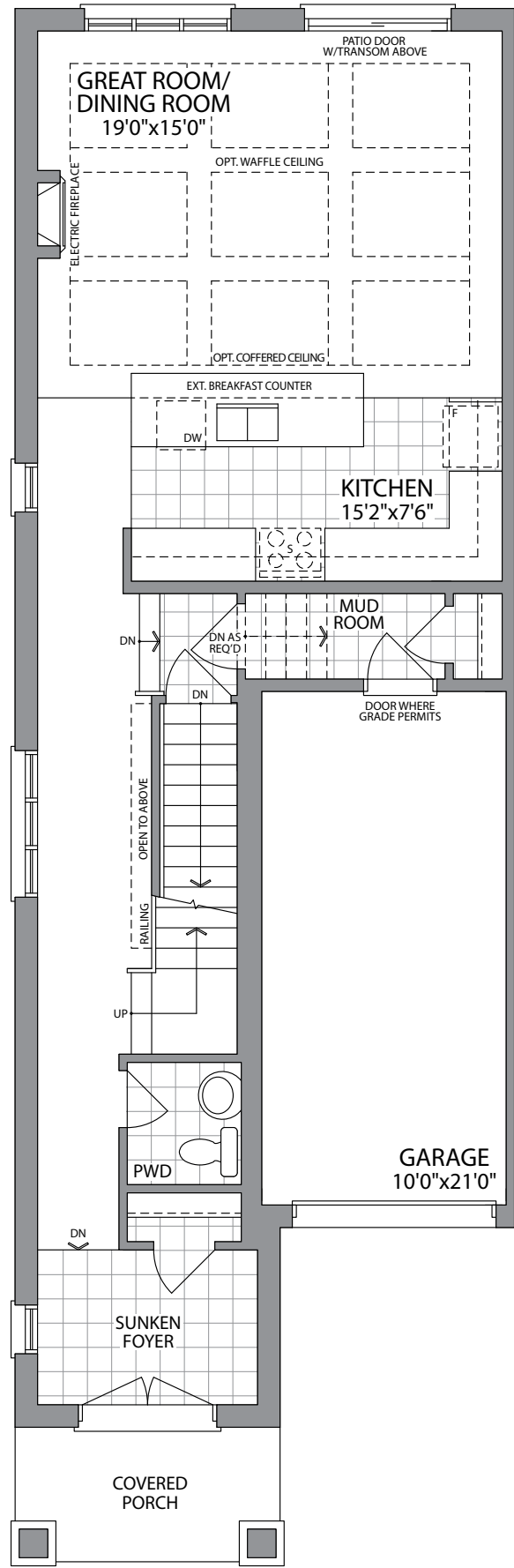
GROUND FLOOR ELEVATION 1C
