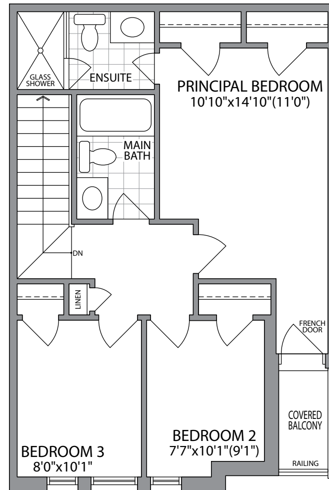
THIRD FLOOR ELEVATION 1
