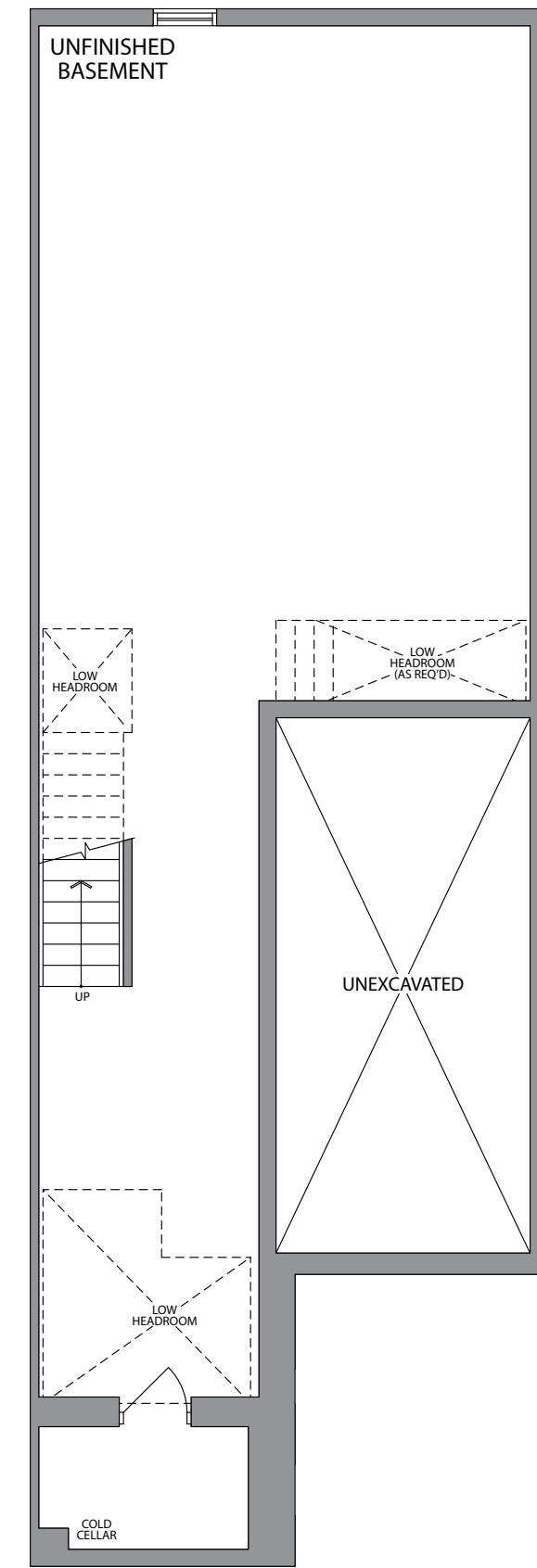
BASEMENT ELEVATION 1 & 2
