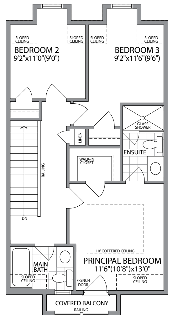
THIRD FLOOR ELEVATION 2
