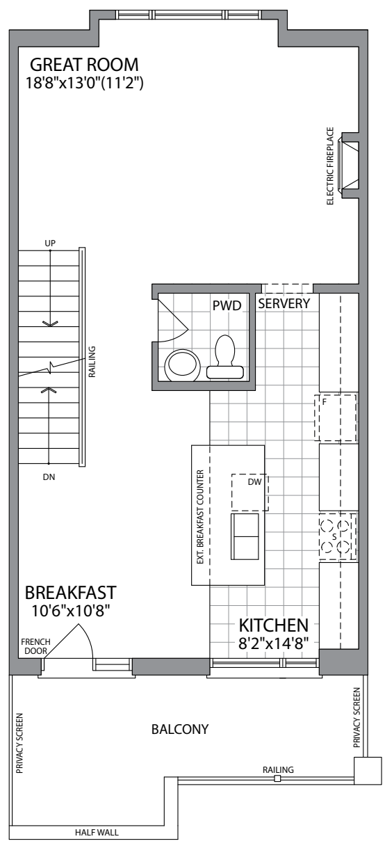
MAIN FLOOR ELEVATION 2
