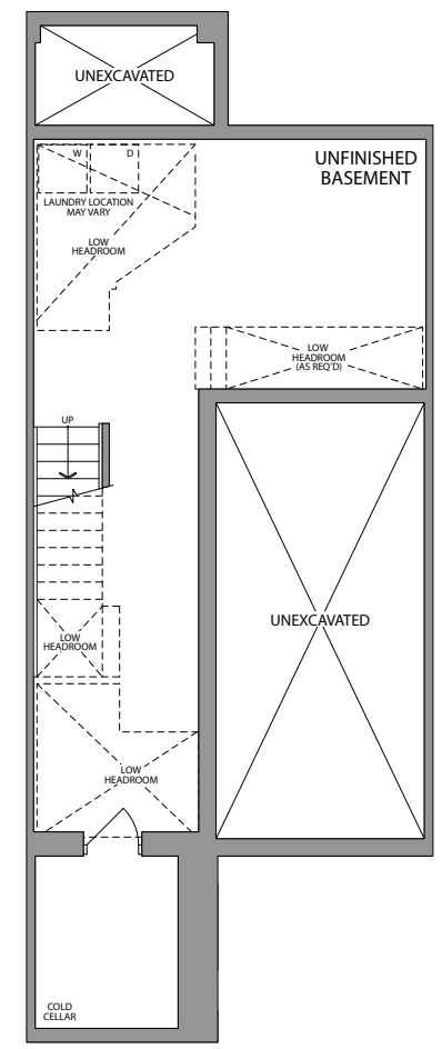
BASEMENT ELEVATION 1 & 2
