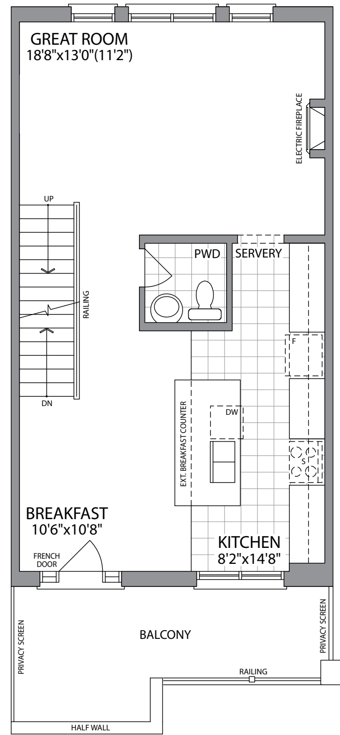
MAIN FLOOR ELEVATION 1
