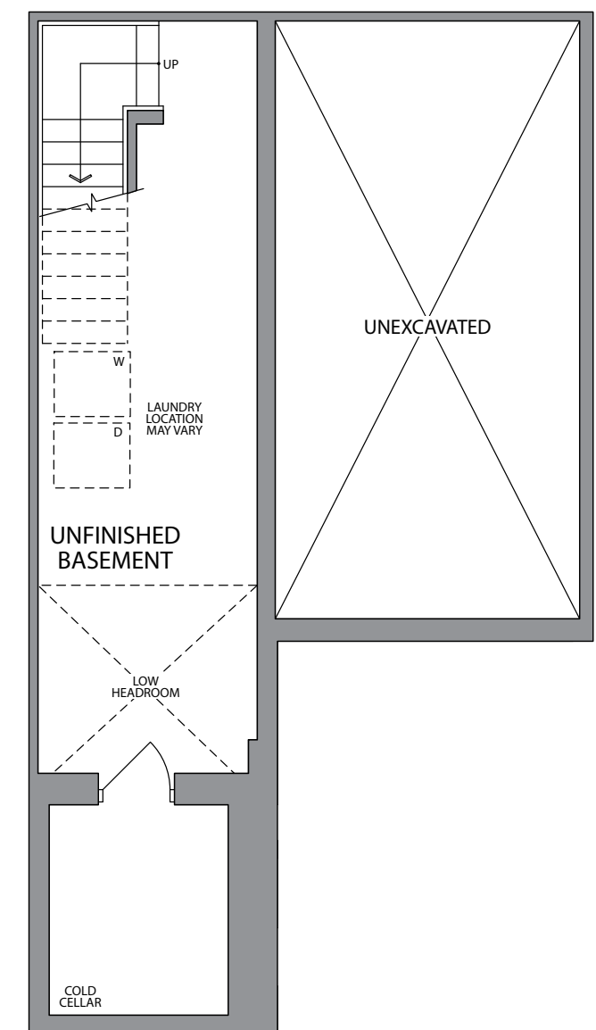
BASEMENT ELEVATION 1 & 2
