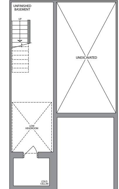
BASEMENT ELEVATION 1
