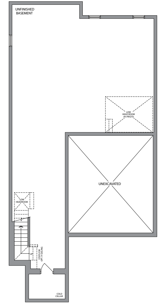
BASEMENT ELEVATION 1
