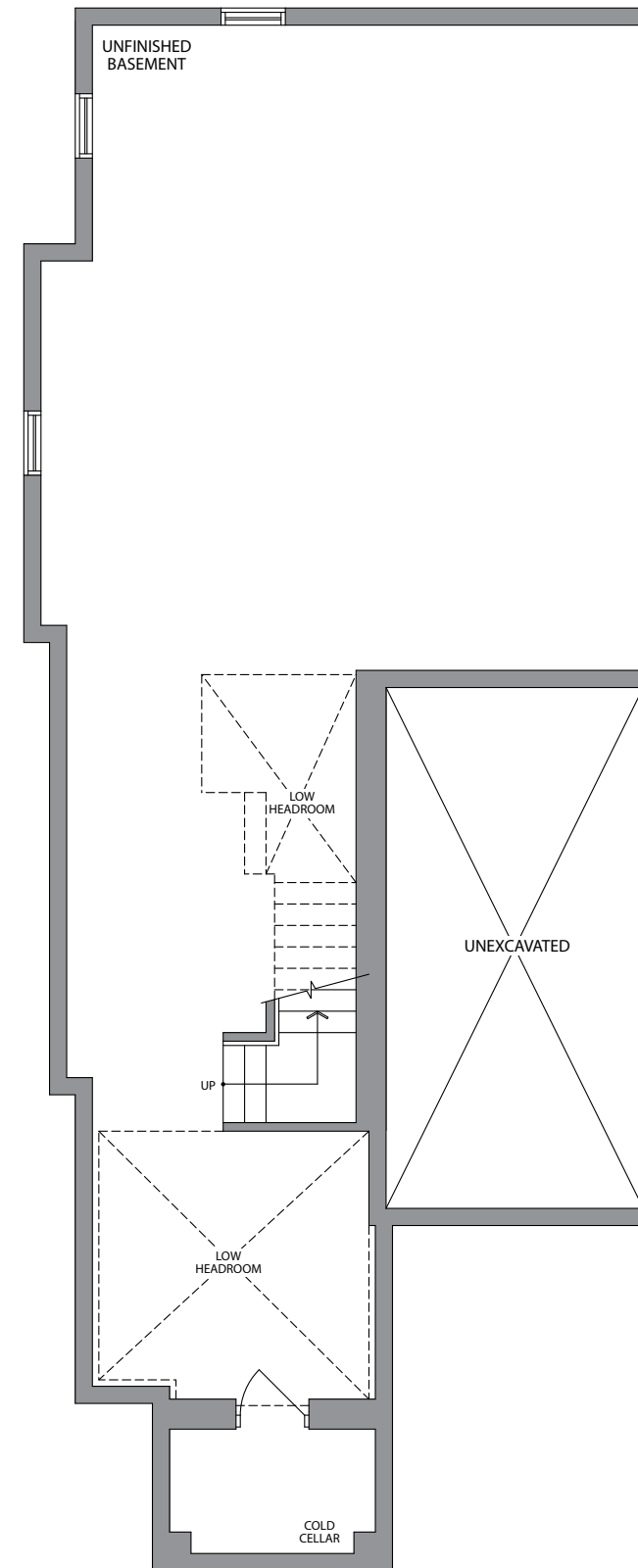
BASEMENT ELEVATION 1C
