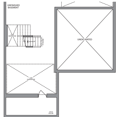
BASEMENT ELEVATION 2
