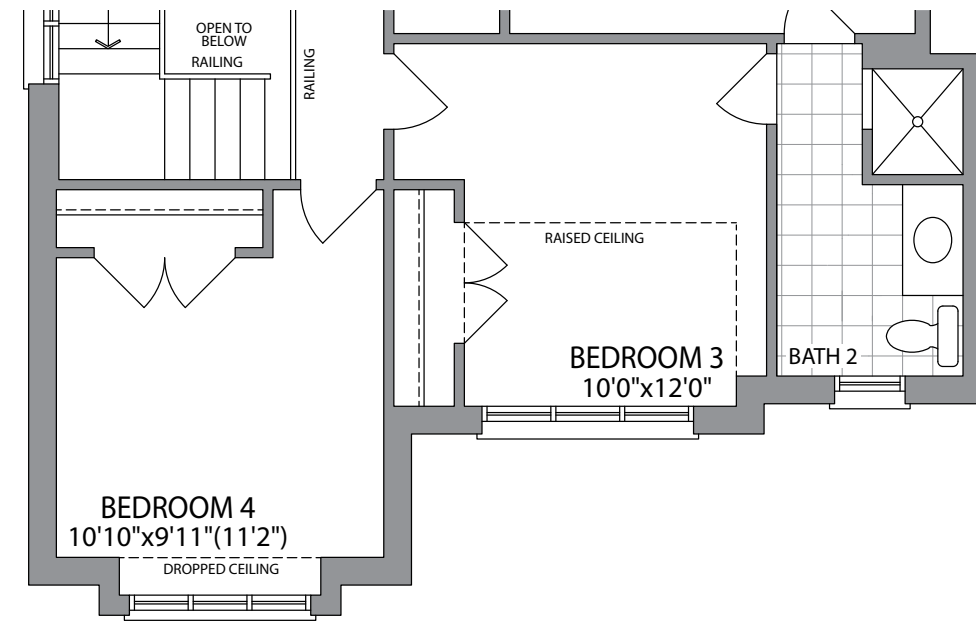
SECOND FLOOR ELEVATION 2
