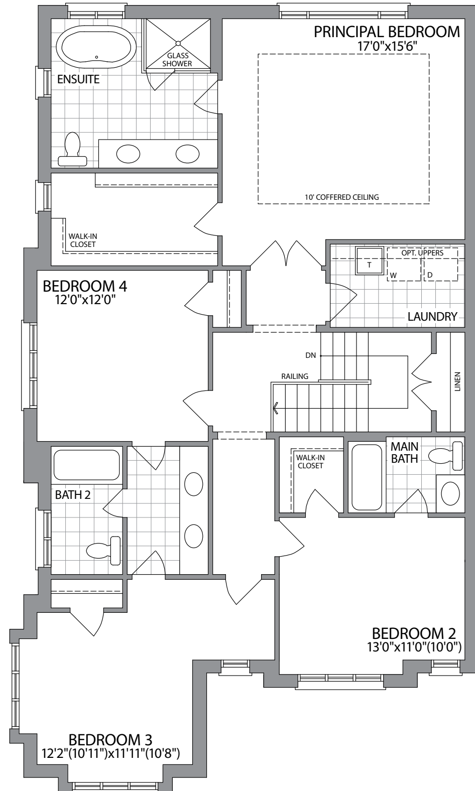
SECOND FLOOR ELEVATION 1C
