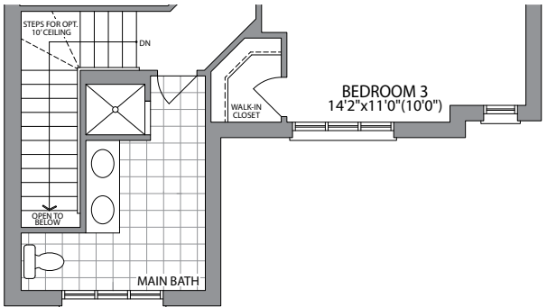
OPT. SECOND FLOOR W/5 BEDROOMS ELEVATION 2
