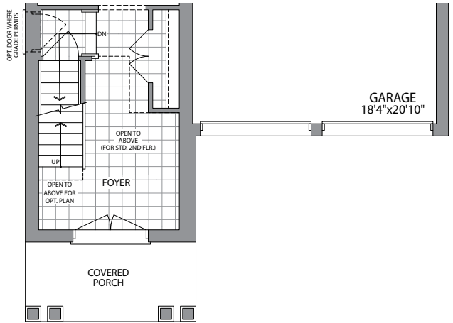
GROUND FLOOR ELEVATION 2
