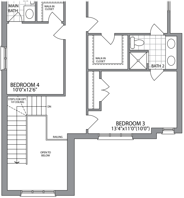
SECOND FLOOR ELEVATION 2
