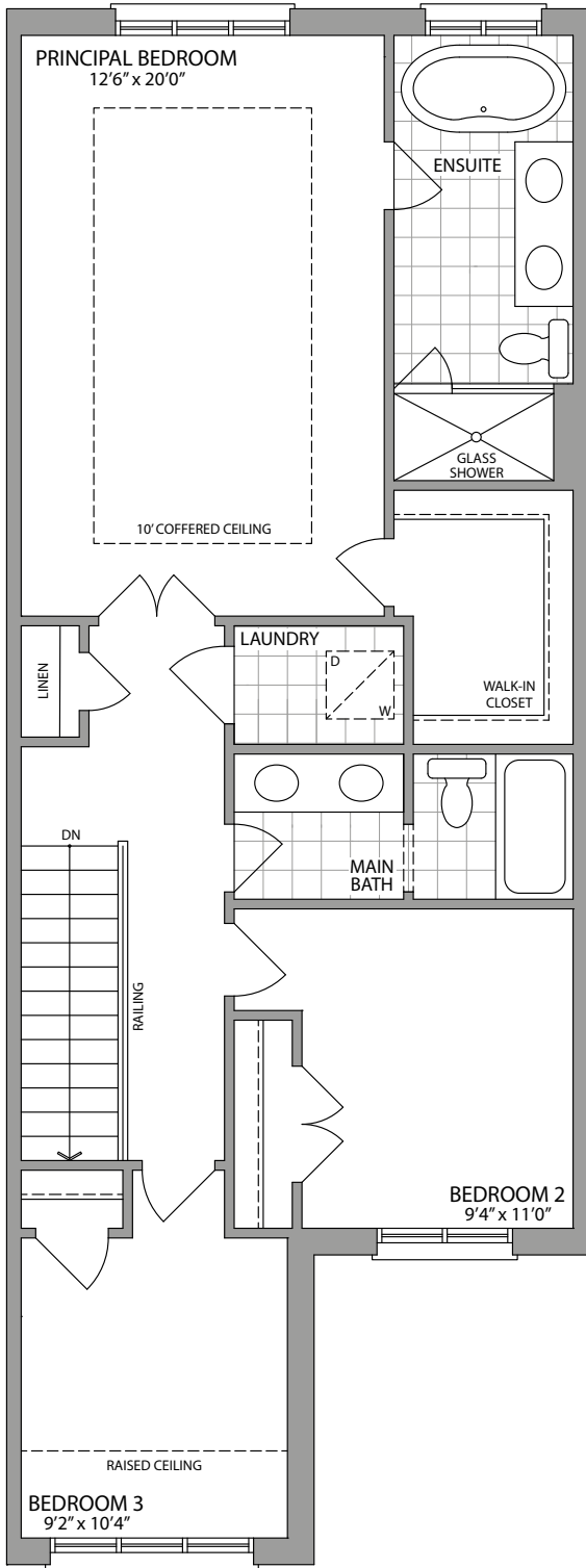
SECOND FLOOR ELEVATION 1
