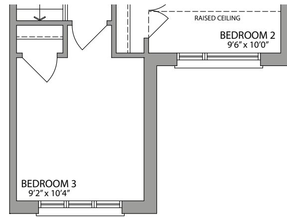
OPT. SECOND FLOOR W/4 BEDROOMS ELEVATION 2
