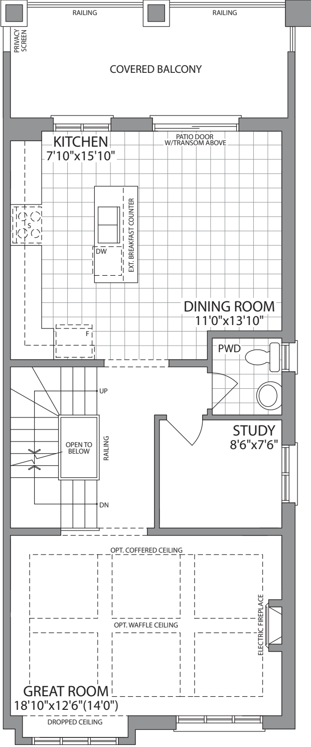
MAIN FLOOR ELEVATION 1C
