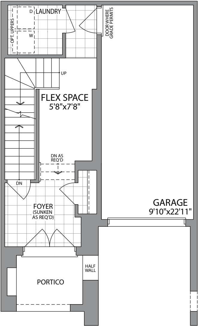
GROUND FLOOR ELEVATION 1
