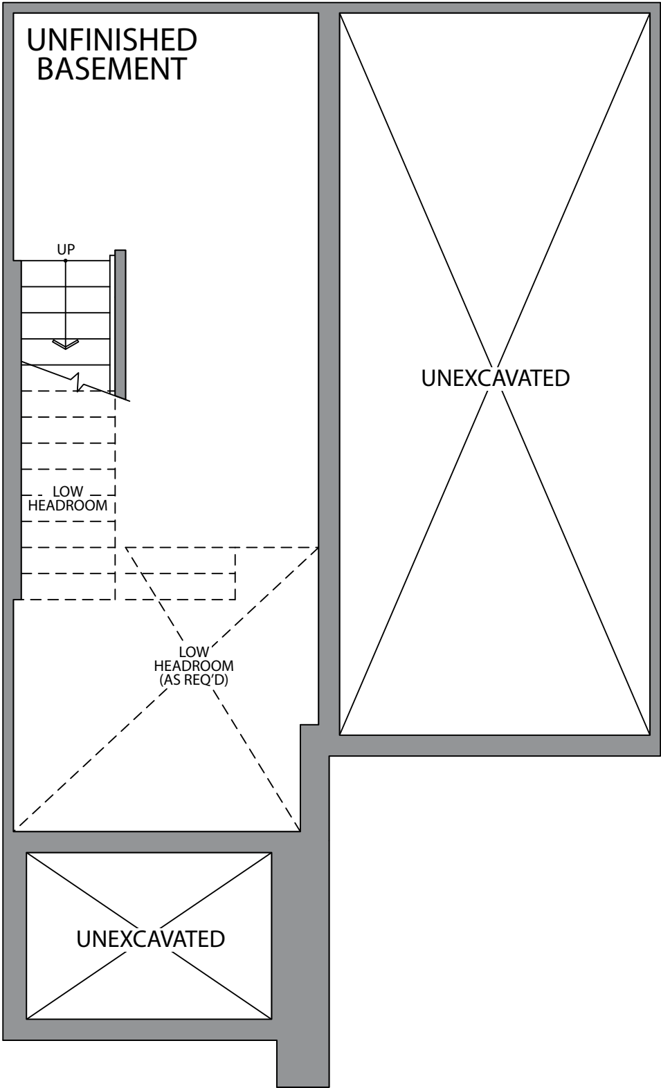
BASEMENT ELEVATION 1
