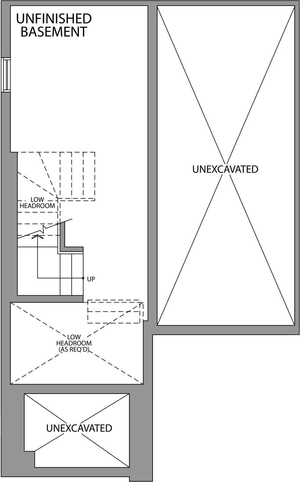
BASEMENT ELEVATION 1C
