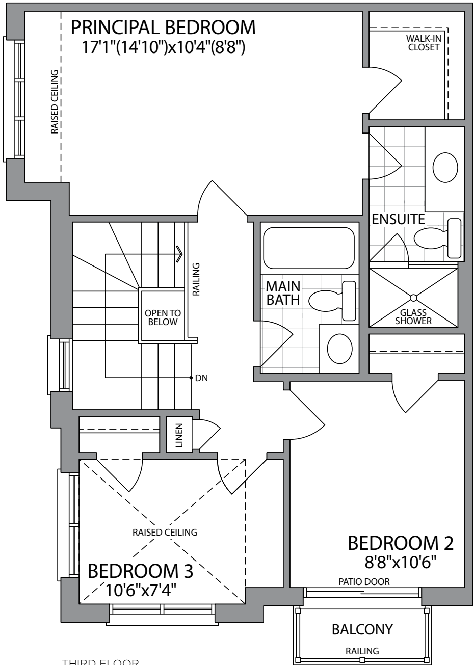
THIRD FLOOR ELEVATION 1C
