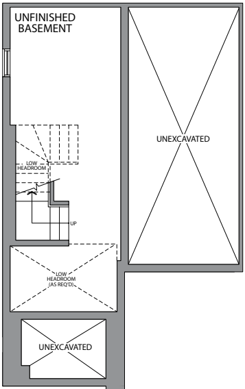
BASEMENT ELEVATION 1C
