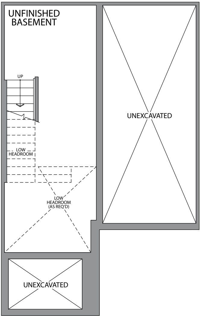
BASEMENT ELEVATION 1 & 2
