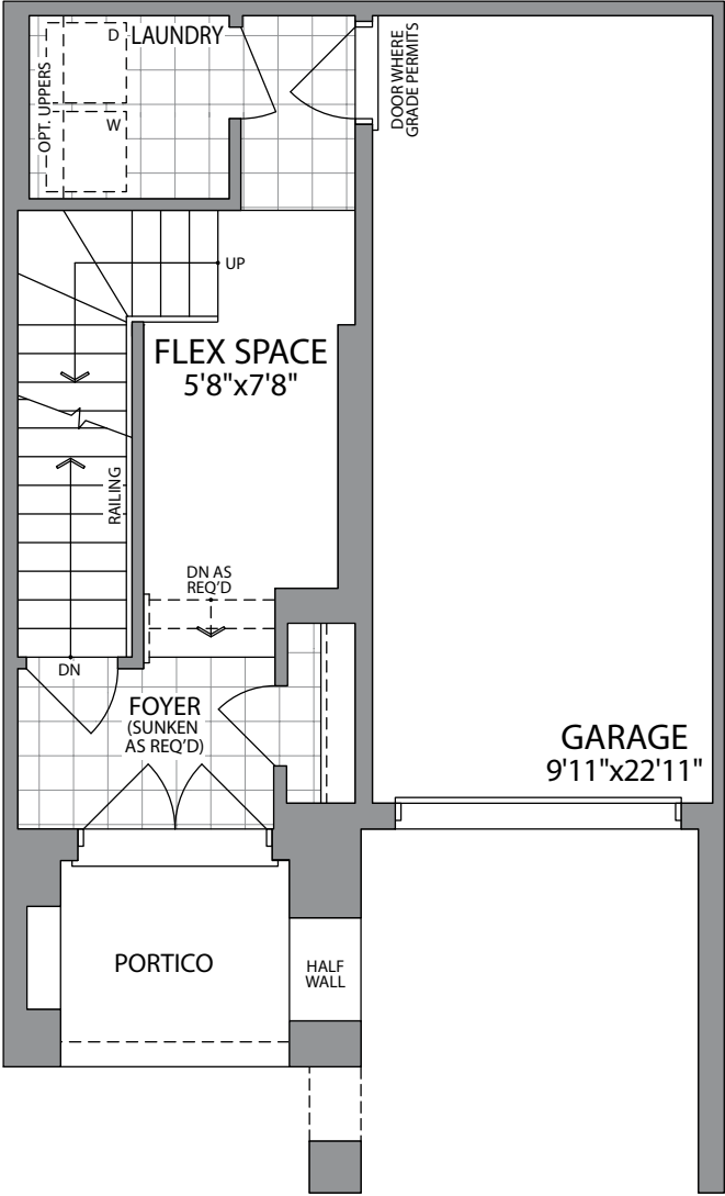
GROUND FLOOR ELEVATION 1 & 2
