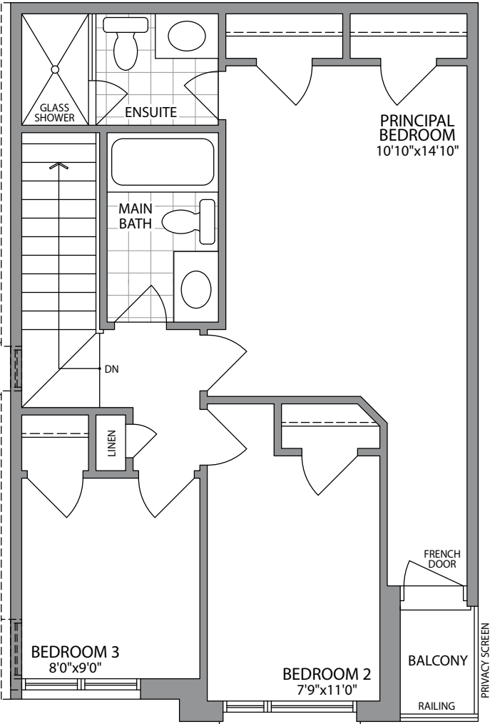
THIRD FLOOR ELEVATION 1/1C
