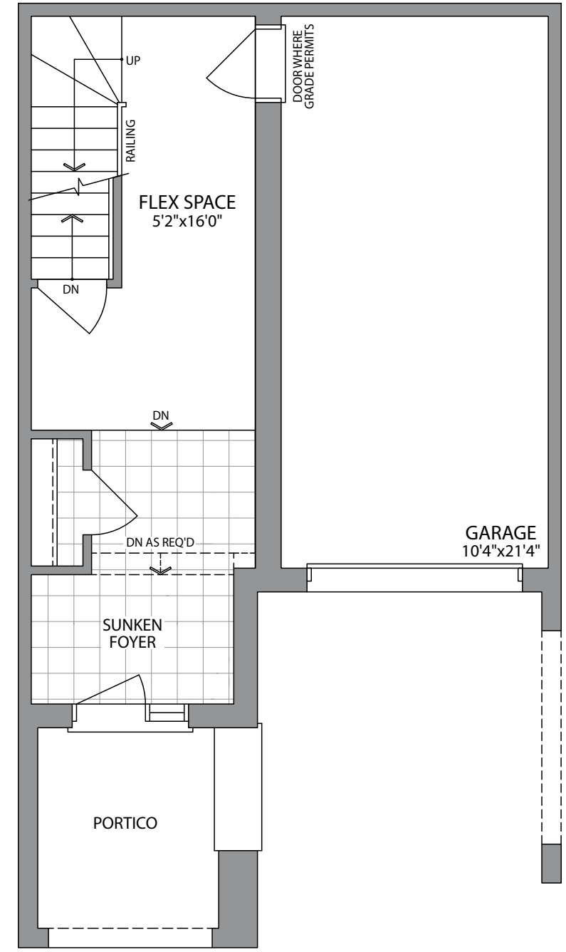
GROUND FLOOR ELEVATION 1
