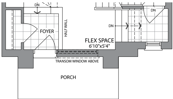
GROUND FLOOR ELEVATION 2
