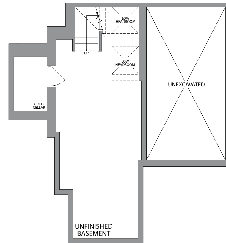
BASEMENT ELEVATION 2C
