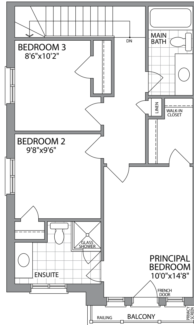
THIRD FLOOR ELEVATION 1C
