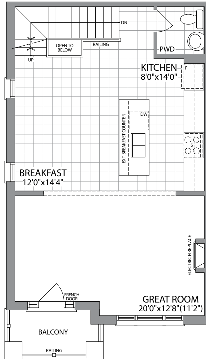
MAIN FLOOR ELEVATION 1C
