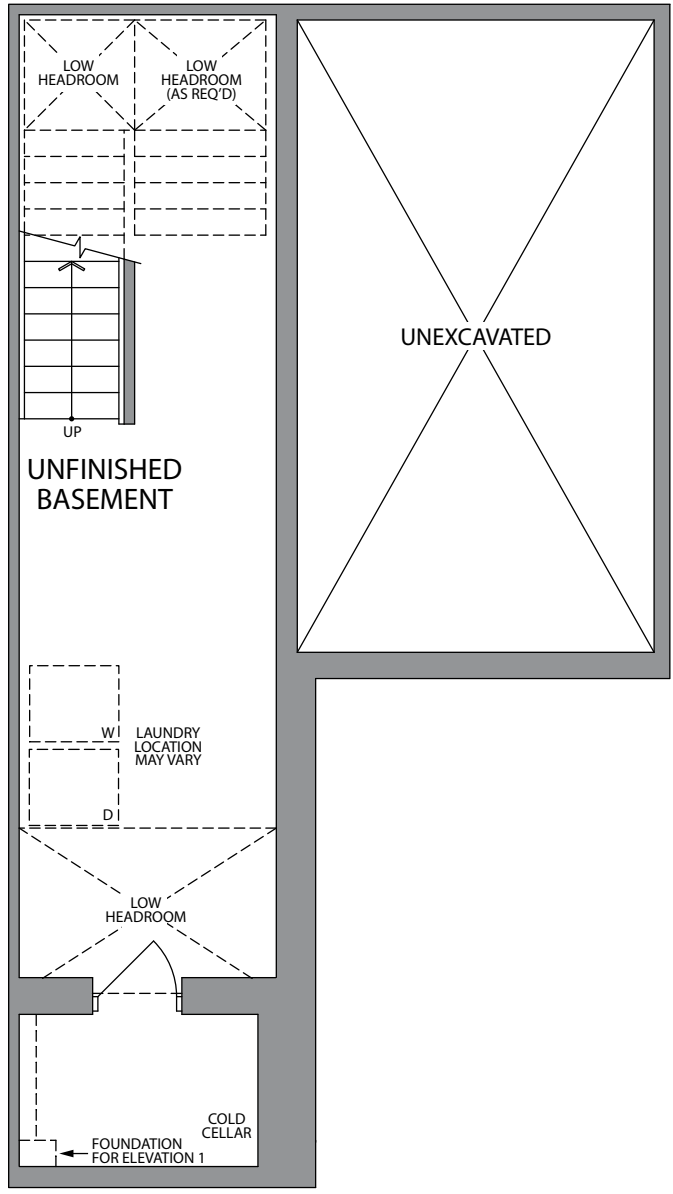
BASEMENT ELEVATION 1 & 2
