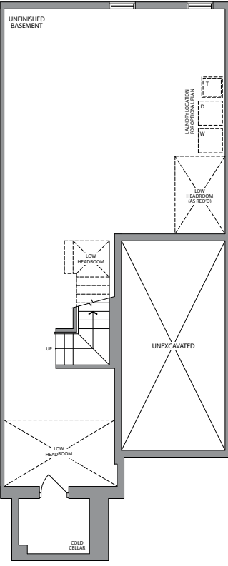
BASEMENT ELEVATION 1
