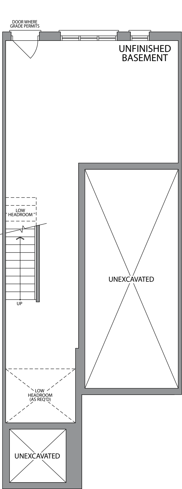
BASEMENT ELEVATION 1
