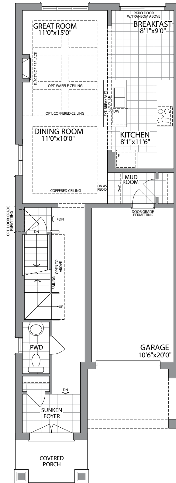
GROUND FLOOR ELEVATION 1C & 2C
