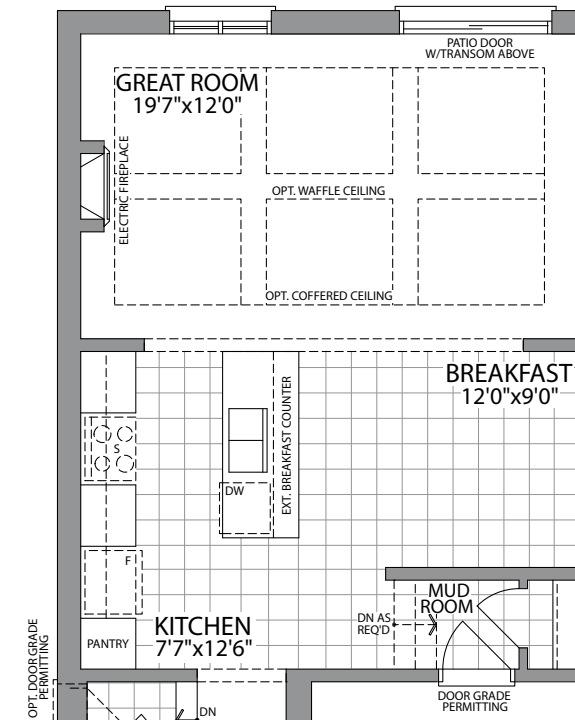
OPT. GROUND FLOOR ELEVATION 1C & 2C
