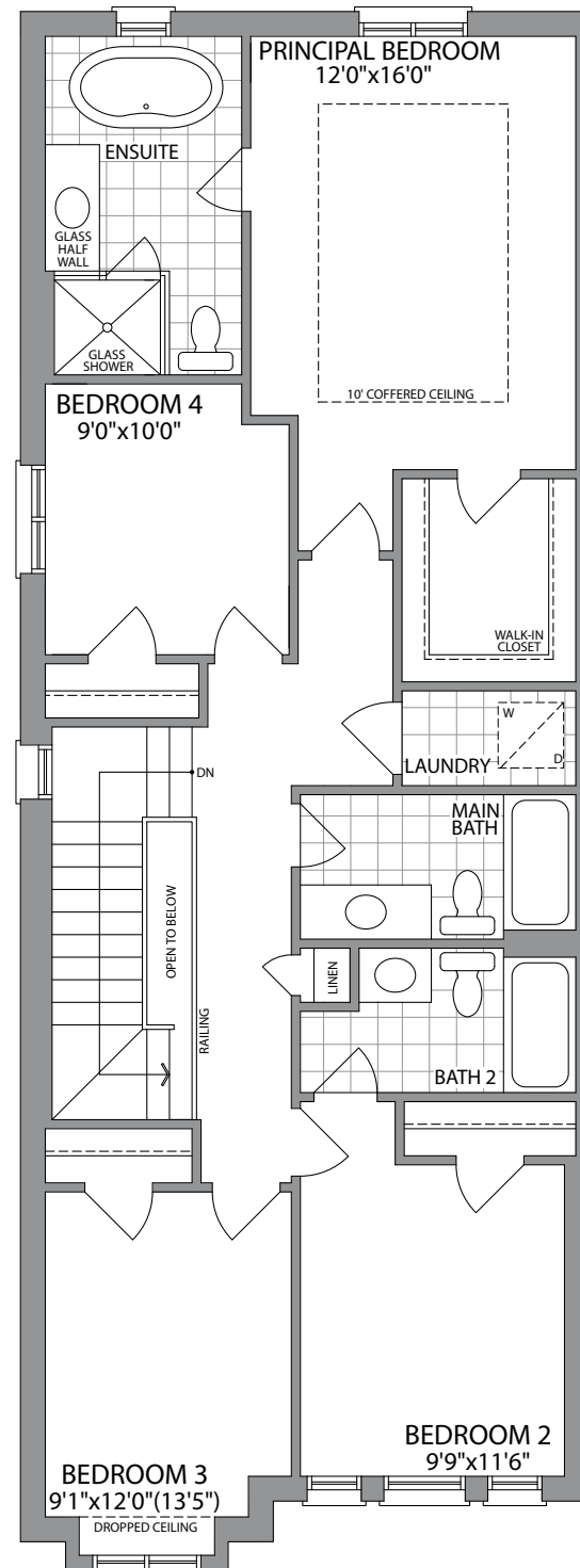
SECOND FLOOR ELEVATION 1C
