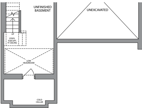
BASEMENT ELEVATION 2
