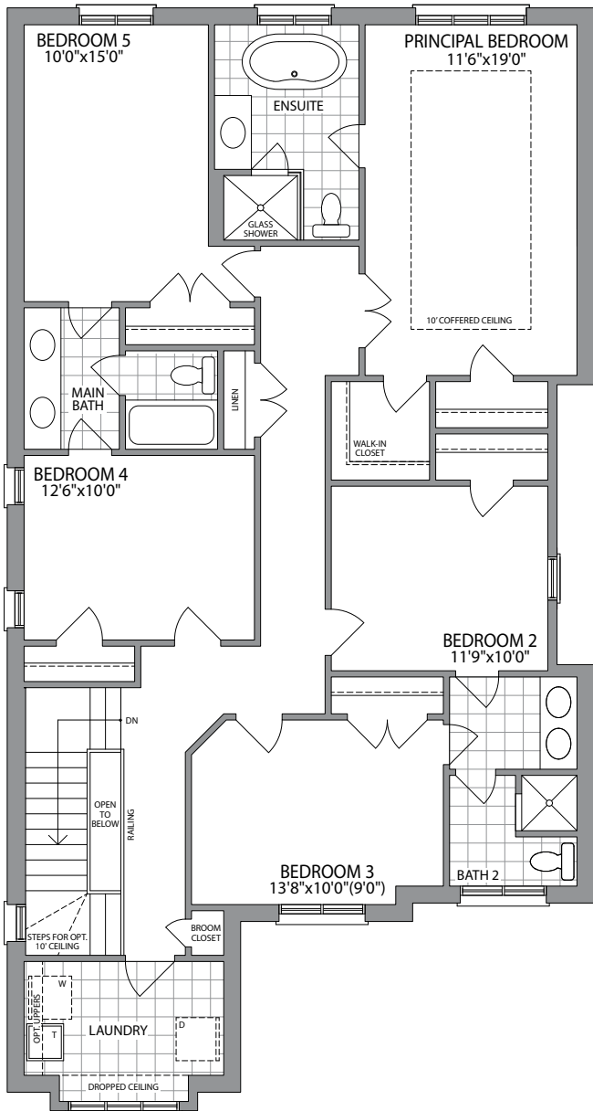
OPT. SECOND FLOOR W/5 BEDROOMS ELEVATION 1
