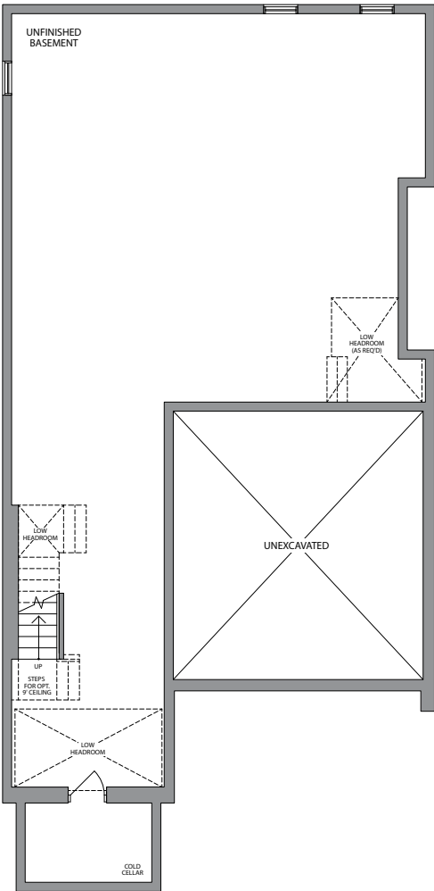
BASEMENT ELEVATION 1
