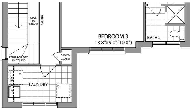
OPT. SECOND FLOOR W/5 BEDROOMS ELEVATION 2
