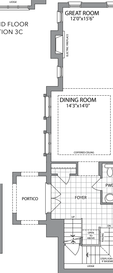
GROUND FLOOR ELEVATION 3C
