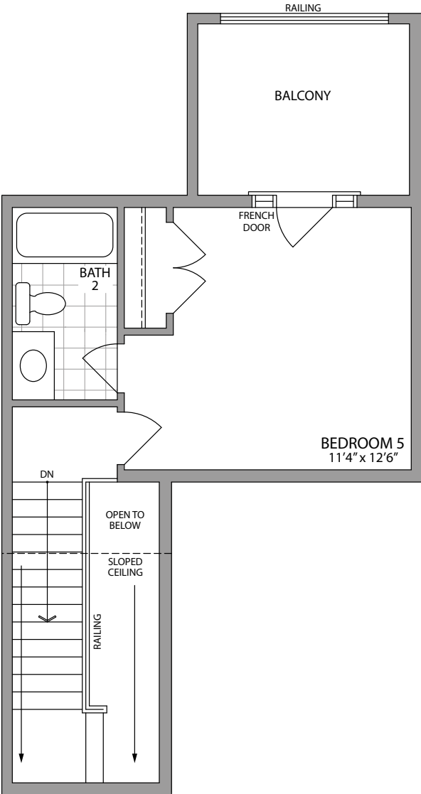
LOFT FLOOR ELEVATION 1 & 2
