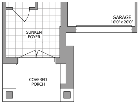
GROUND FLOOR ELEVATION 2
