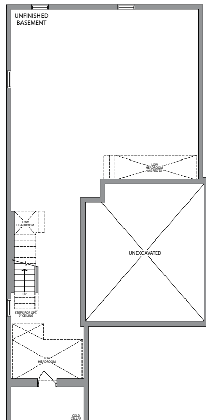
BASEMENT ELEVATION 1 & 2
