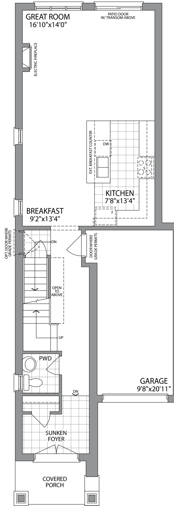
GROUND FLOOR ELEVATION 1C
