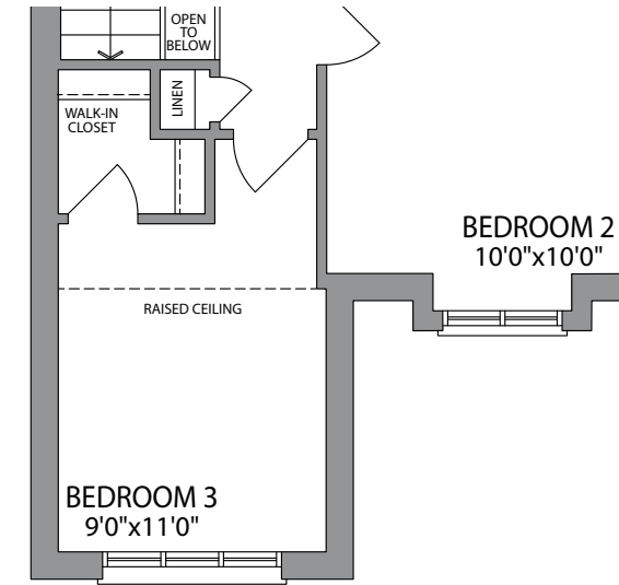
SECOND FLOOR ELEVATION 2C
