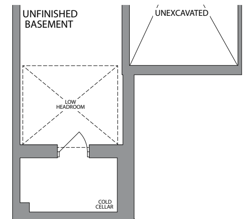
BASEMENT ELEVATION 2C
