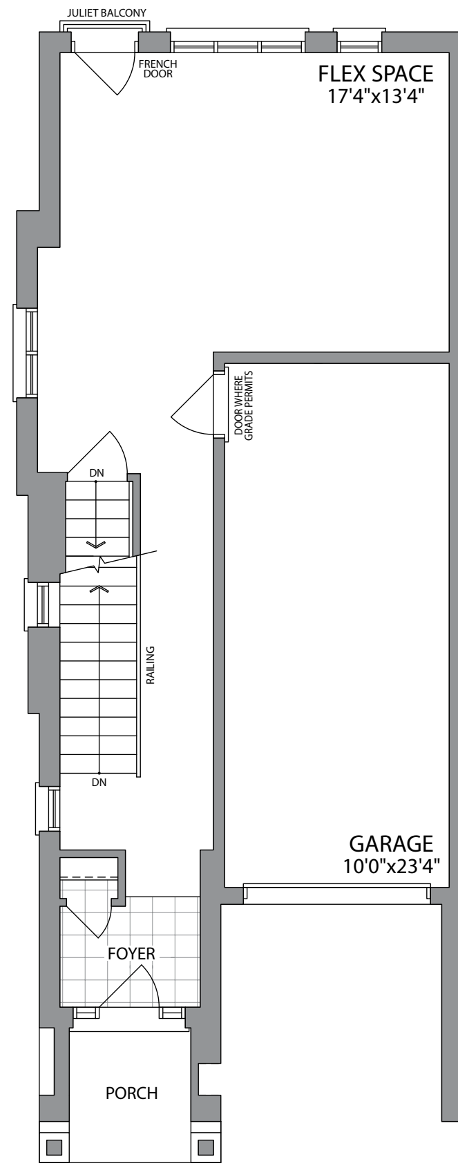
GROUND FLOOR ELEVATION 1C
