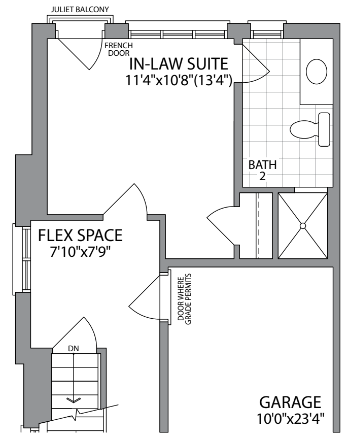
OPT. GROUND FLOOR W/IN-LAW SUITE ELEVATION 1C
