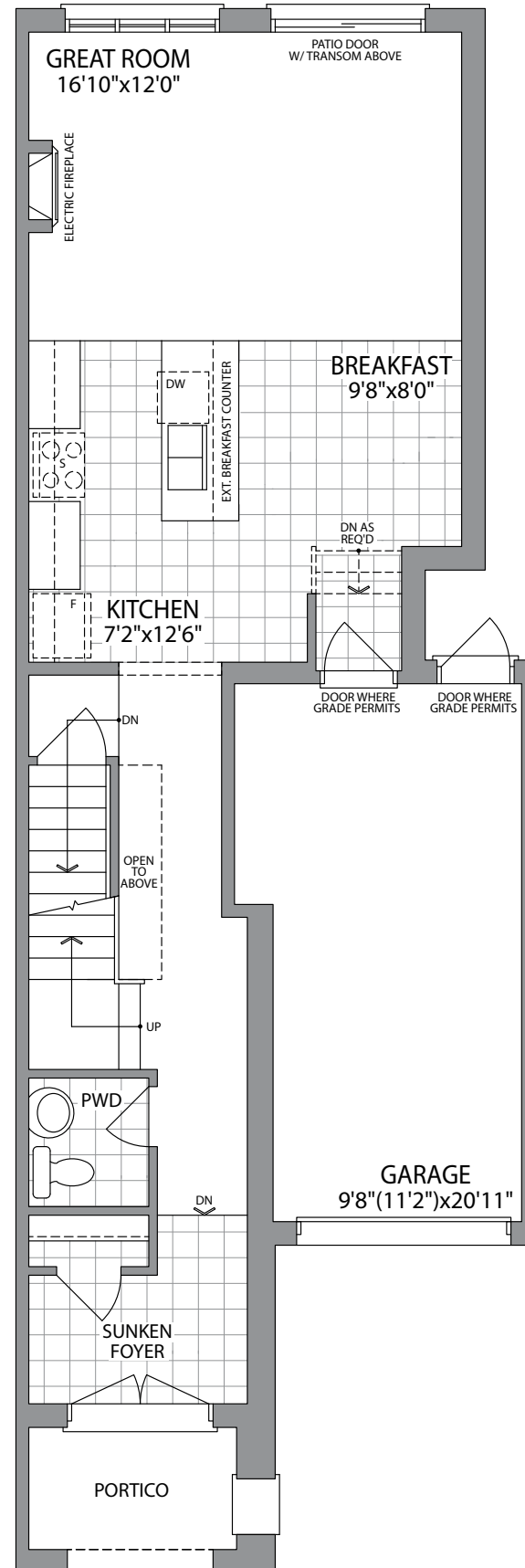
GROUND FLOOR ELEVATION 1
