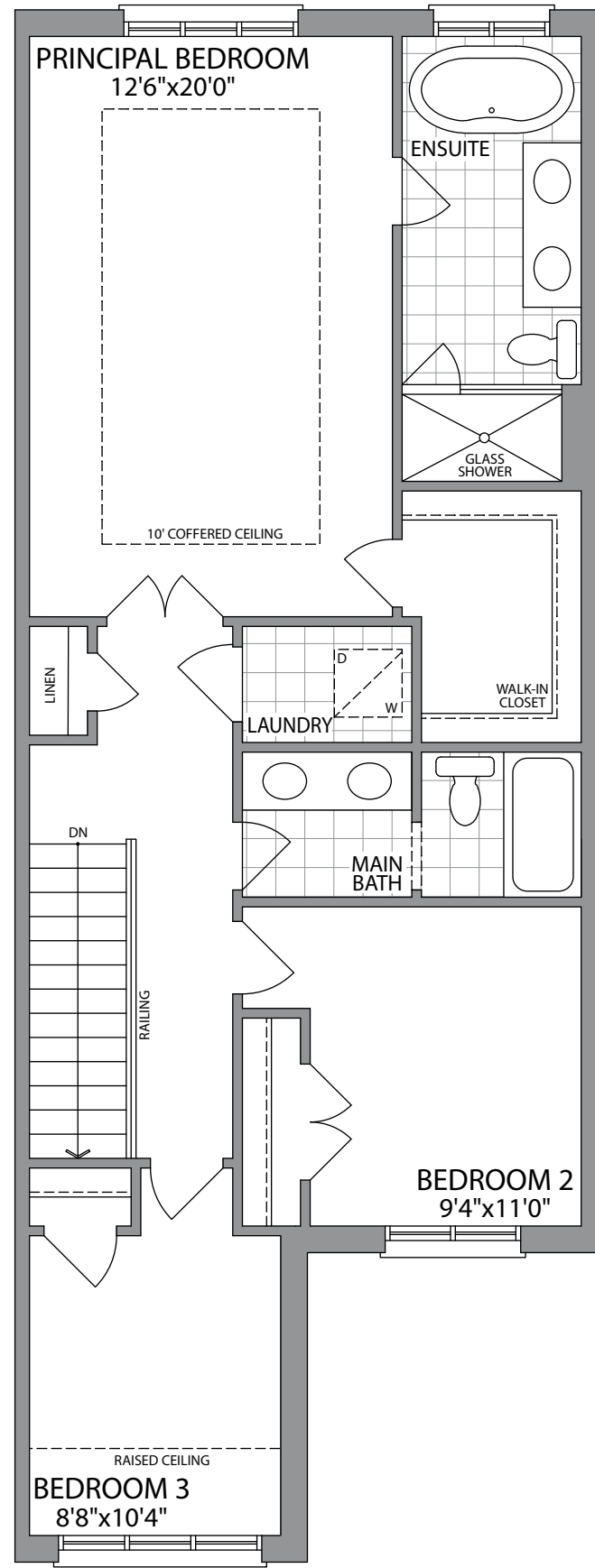
SECOND FLOOR ELEVATION 1
