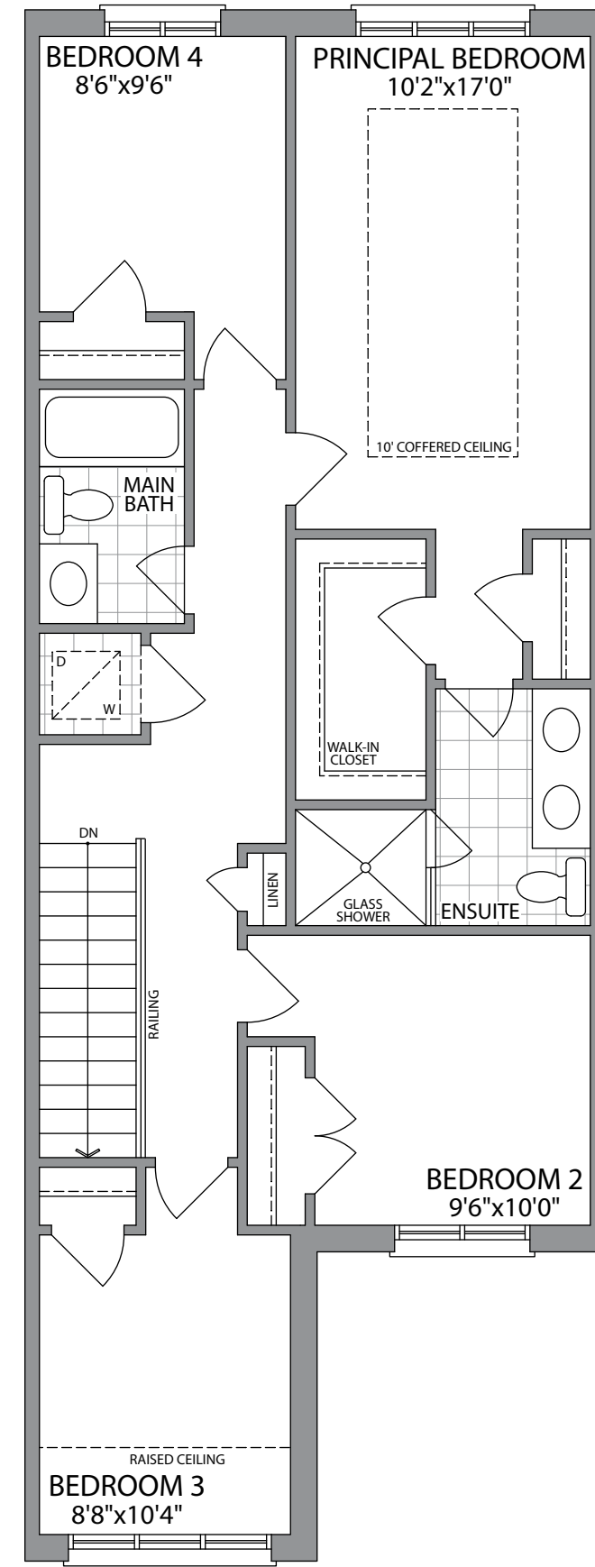
OPT. SECOND FLOOR W/4 BEDROOMS ELEVATION 1
