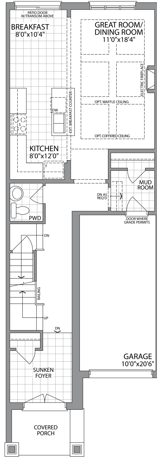
GROUND FLOOR ELEVATION 1
